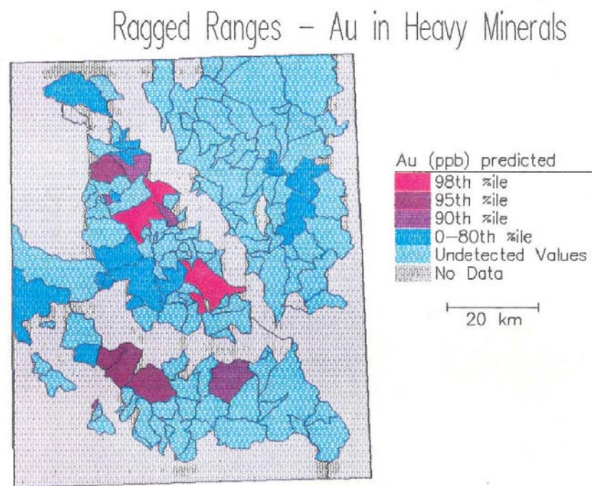
Figure 4.5b: Ragged Ranges, Au in HMC using MLE – Predicted Data
