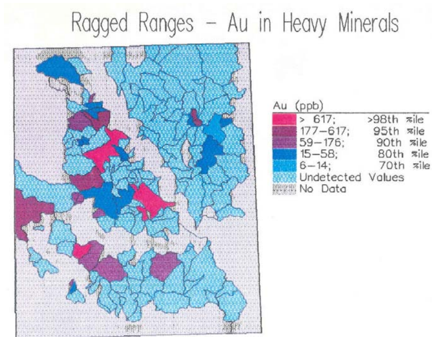
Figure 4.5a: Ragged Ranges, Au in HMC using MLE – Raw Data
