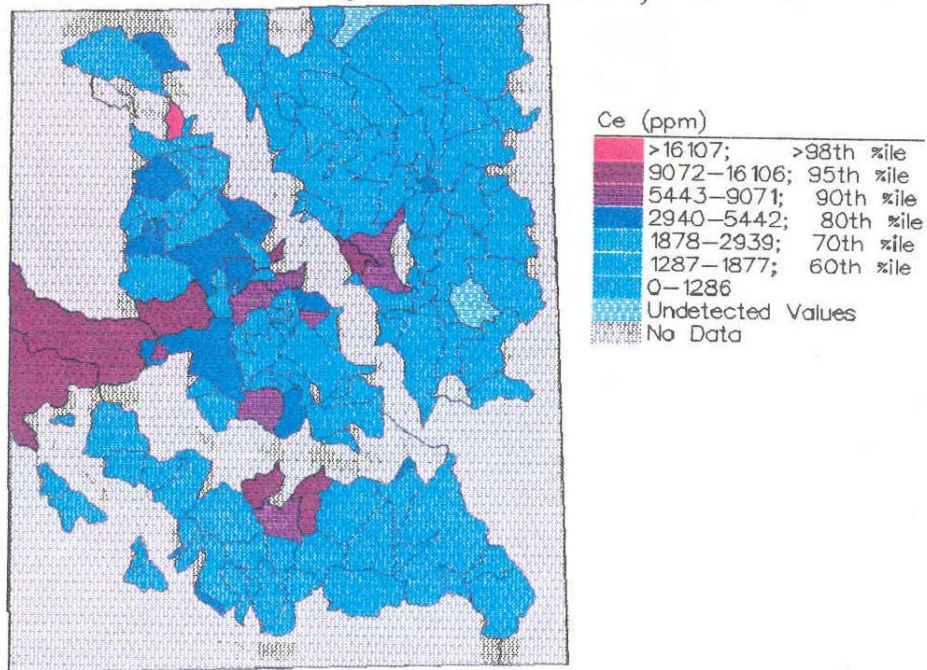
Figure 4.21a: Ragged Ranges, Ce in HMC using MLE – Raw Data
