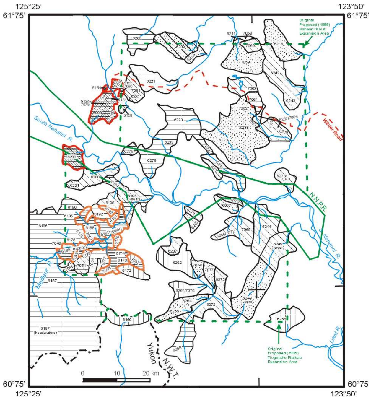
Figure 4.41a: NK/TP Mineral Potential Summary Map (for legend, see Figure 4.40a)
