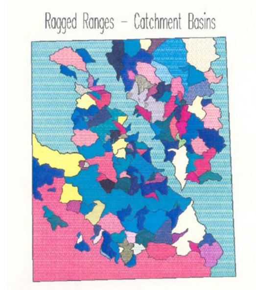
Figure 4.4: Catchment basins for Ragged Ranges
