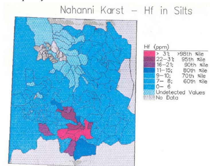
Figure 4.11a: Nahanni Karst, Hf in silt using MLE – Raw Data
