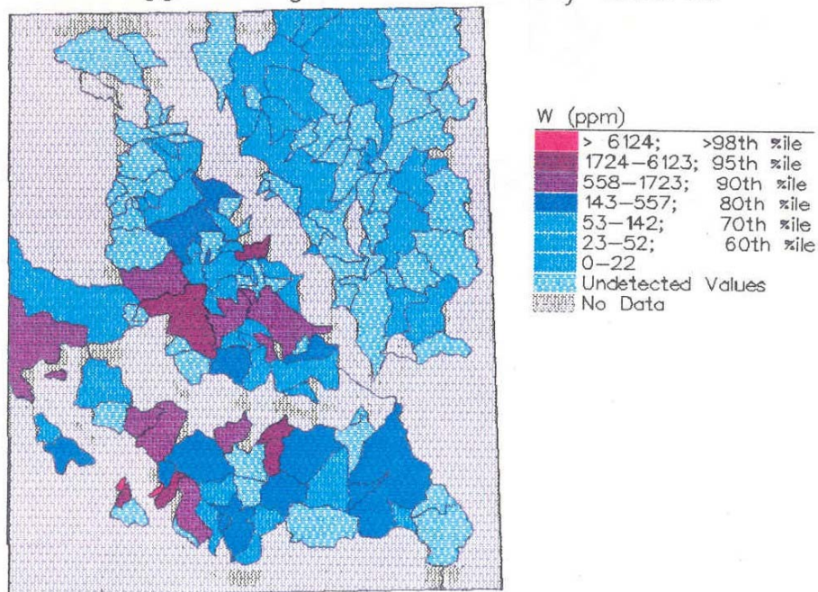
Figure 4.7a: Ragged Ranges, W in HMC using MLE – Raw Data
