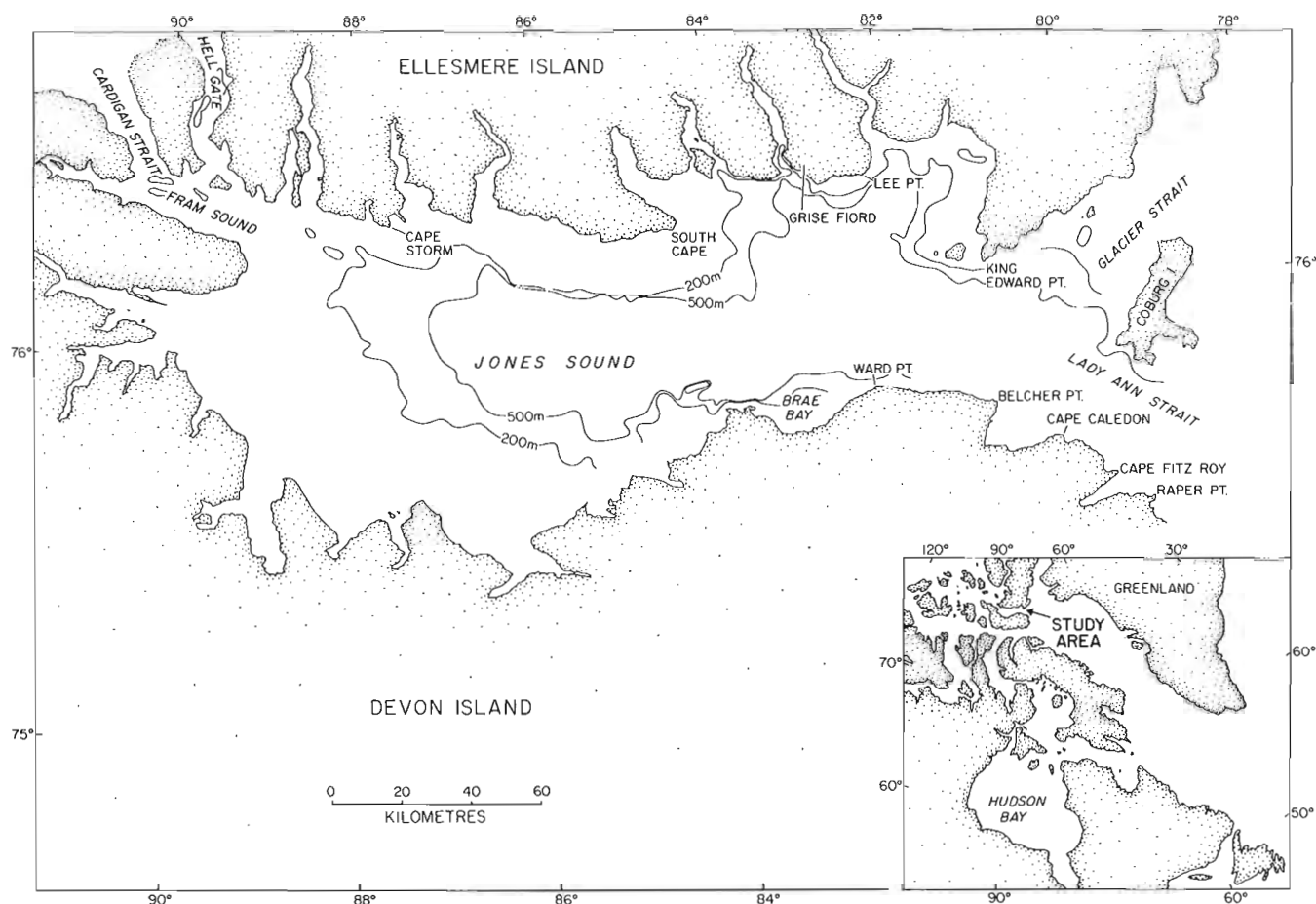
Figure 49.1. Index map of Jones Sound study area.
