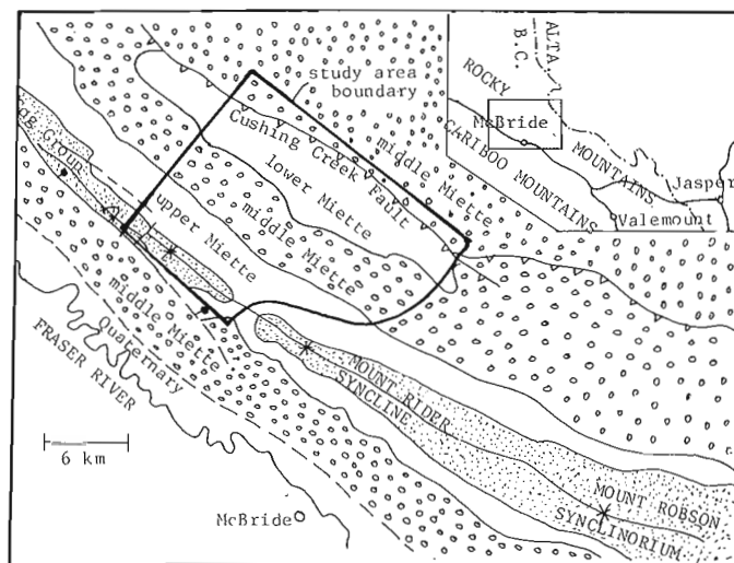
Figure 56.1. Location map and generalized geology map (after GSC Map 1356A).
