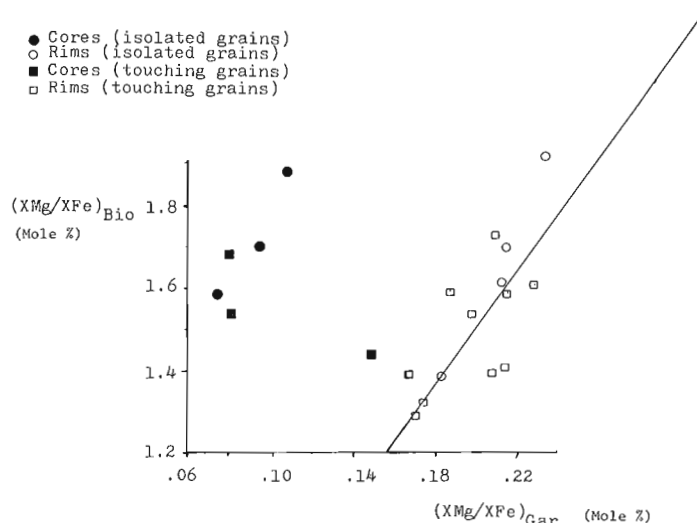
Figure 20.7. (\text{XMg}/\text{XFe})_{\text{gar}} vs (\text{XMg}/\text{XFe})_{\text{bio}} plot. Cores and rims are plotted separately and a distinction is made between isolated grains and grains in contact with each other (garnet-biotite). The line shown passes through the origin and gives an average K_d (inverse of slope) for rims of grains.
