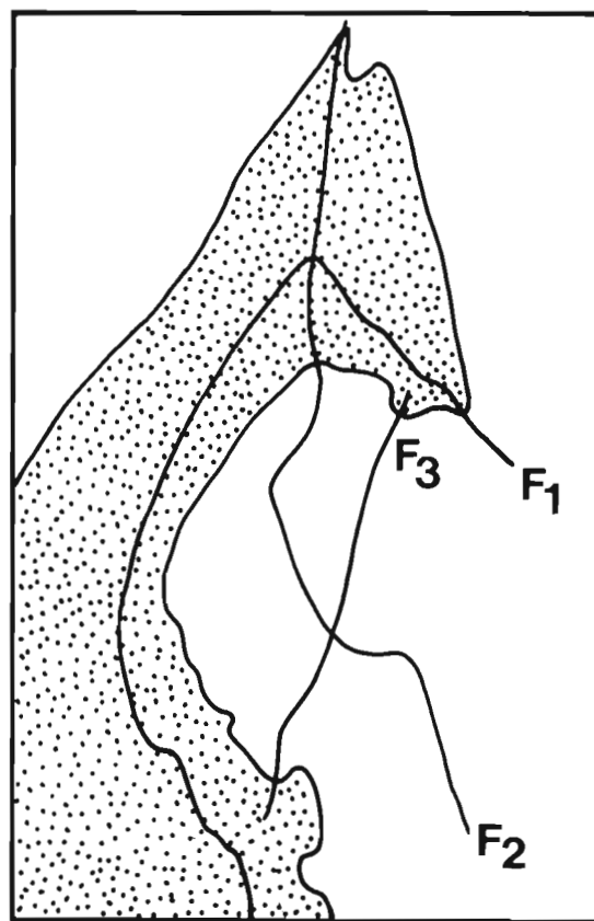
b) Axial traces of folds in Figure 25.3a; F 3 is coaxial with the folds of basement.
