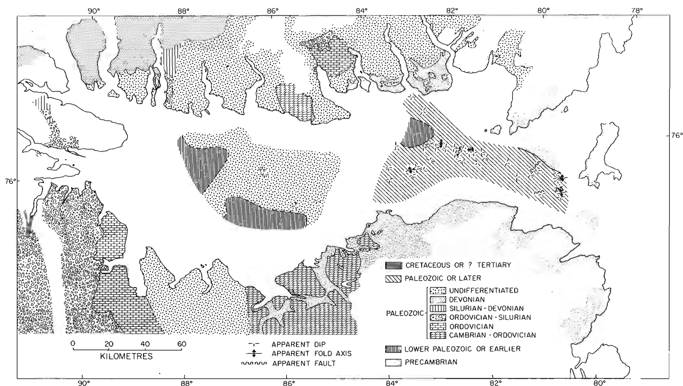
Figure 49.6. Chart showing preliminary interpretation of bedrock geology offshore in Jones Sound based on seismic reflection and magnetometer data together with the adjacent onshore geology (after Frisch, 1983; Fortier et al., 1963).
