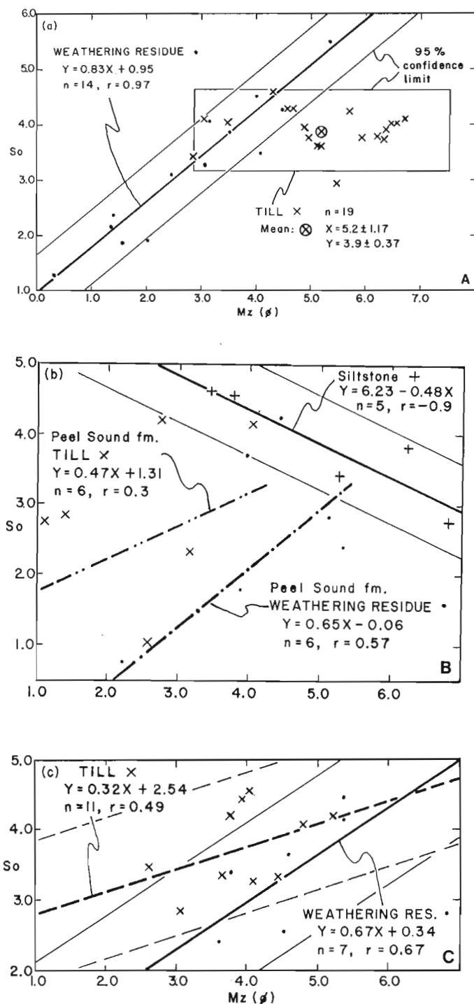
Figure 46.3. Regression curves of sorting coefficients on mean grain sizes of diamictons derived from various rocks: A. crystalline rocks; B. clastic rocks; C. carbonate rocks. The thick lines are regression curves and the corresponding parallel thin lines represent the 95% confidence limits of these curves, or two standard errors. For the till in 3A, confidence limits are taken as two standard deviations of both X and Y.
