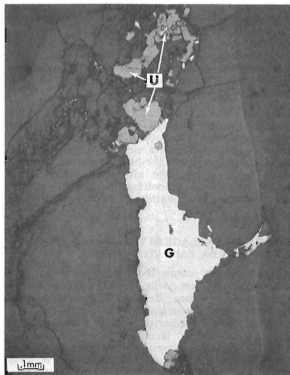
Figure 5.19. Guanajuatite (\text{Bi}_2\text{Se}_3) – (G) and uraninite (U) from a fracture filling associated with aplitic rocks intruding arkosic conglomerate, Otish Mountains area, Quebec. Photomicrograph, reflected light.
