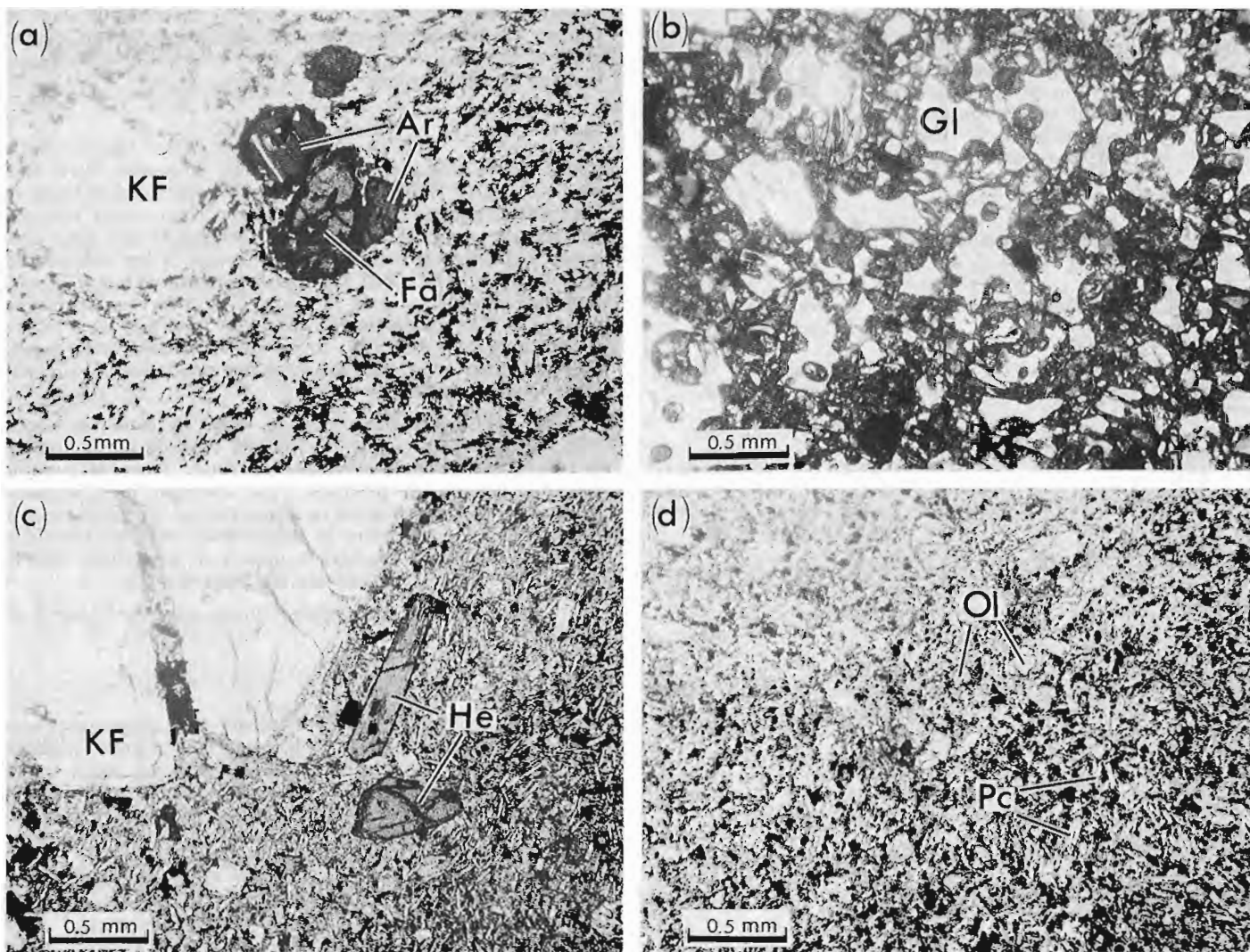
Figure 1.4. Photomicrographs: (a) porphyritic comendite, unit 4; (b) vitric tuff, unit 6; (c) porphyritic trachyte, unit 7; (d) aphyric hawaiite, unit 10. (Gl-glass, Pc-plagioclase, KF-alkali feldspar, ol-olivine, Fa-fayalite, He-hedenbergite, Ar-arfvedsonite)
