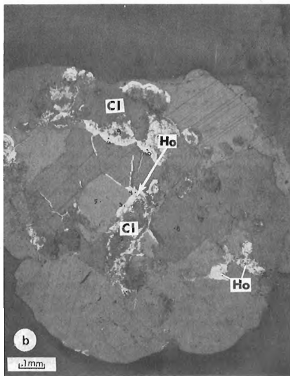
Figure 5.20a,b. Curite (?) (\text{Pb}_2\text{U}_5\text{O}_{17} \cdot 4\text{H}_2\text{O}) (Ct) and hollandite (\text{BaMn}_8\text{O}_{16}) (Ho) associated with clay (Cl) and dolomite (Do) from a carbonate vein associated with rhyolitic rocks intruding quartz-pebble conglomerate, Otish Mountains, Quebec. Photomicrographs, (a) transmitted light, (b) reflected light.
