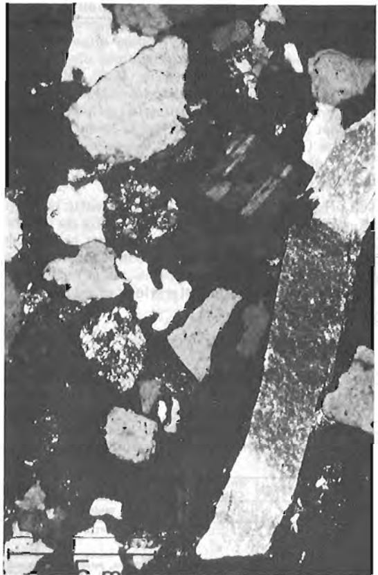
Figure 47.6. Large muscovite grain in host rock sandstone. Bar scale is 0.5 mm.
