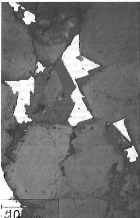
Figure 47.4. Straight-edge contacts between galena and silica overgrowths on detrital quartz grains. Bar scale is 100 \mu\text{m} .
