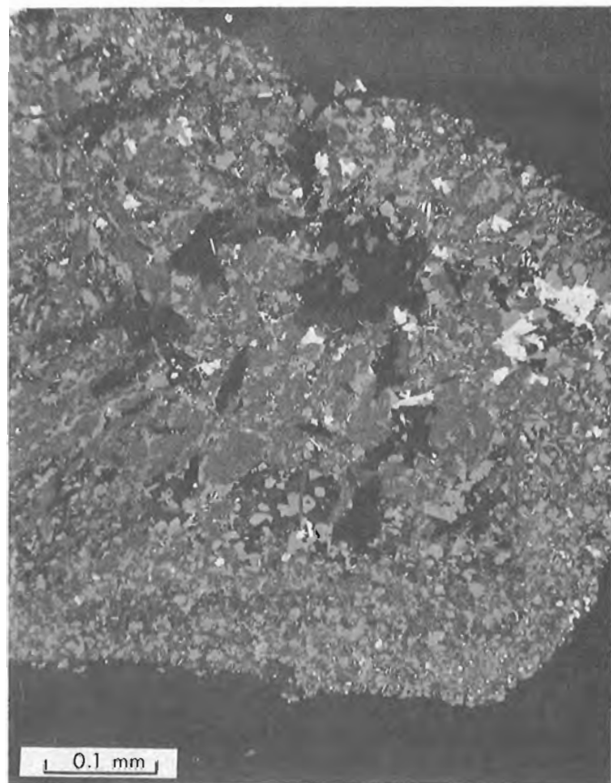
Figure 5.6. A grain of intergrown Ti-U-Si phase (dark grey) with anatase/rutile (light grey) and galena (white) in quartz-pebble conglomerate from the Panel mine, Elliot Lake, Ontario. Photomicrograph, reflected light.
