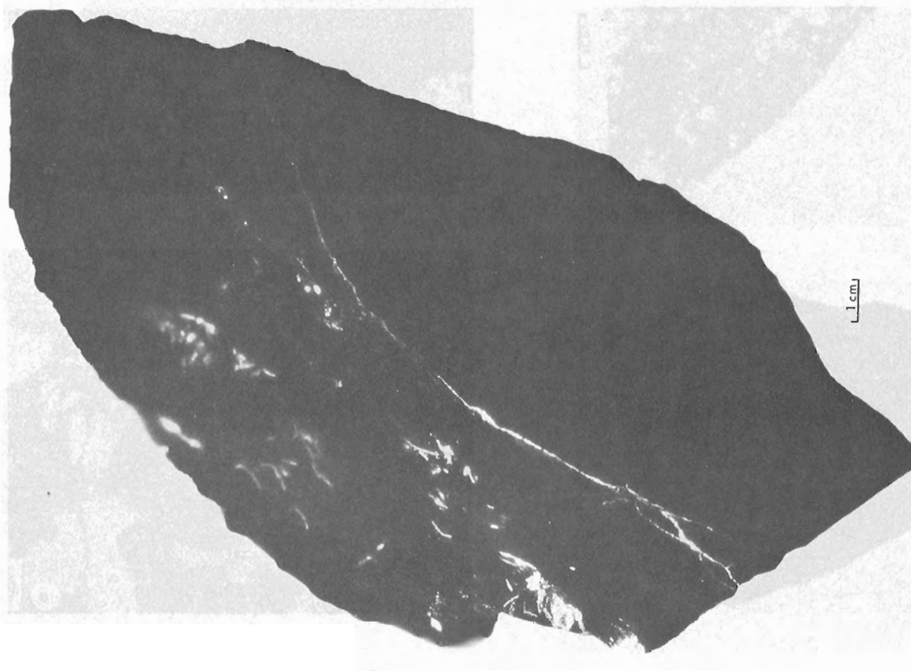
Figure 5.9. Autoradiograph of a ferruginous rock mineralized by pitchblende (white streaks); Black Sturgeon Lake uranium occurrence, Ontario.
