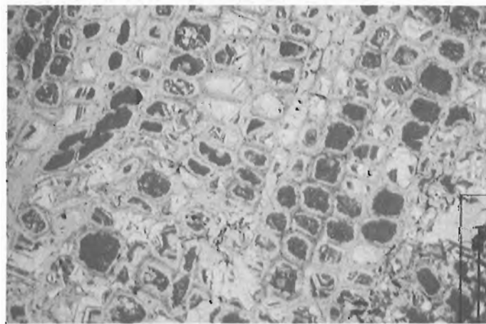
Figure 47.13. Pyrite (light grey) and sphalerite (dark) within wood cells; galena (white) replaces cell walls. Bar scale is 100 \mu m.
