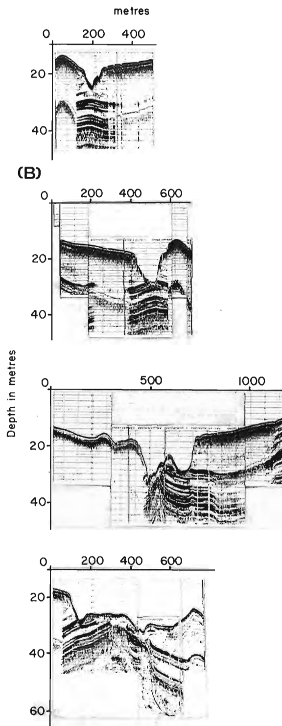
Figure 76.9. Profiles across a trench created by subaqueous mudflow in the north part of Lake Timiskaming. A. Location of the trench on the profile extending to Mann Island; note surface sediments draped over "pillars" of laminated sediment thought to have been deposited in crevasses in stagnant ice. B. Profiles of the mudflow trench from the east end (top) to the west end (bottom). Note diapirism and general disturbance of older proglacial sediment beneath the trench.
