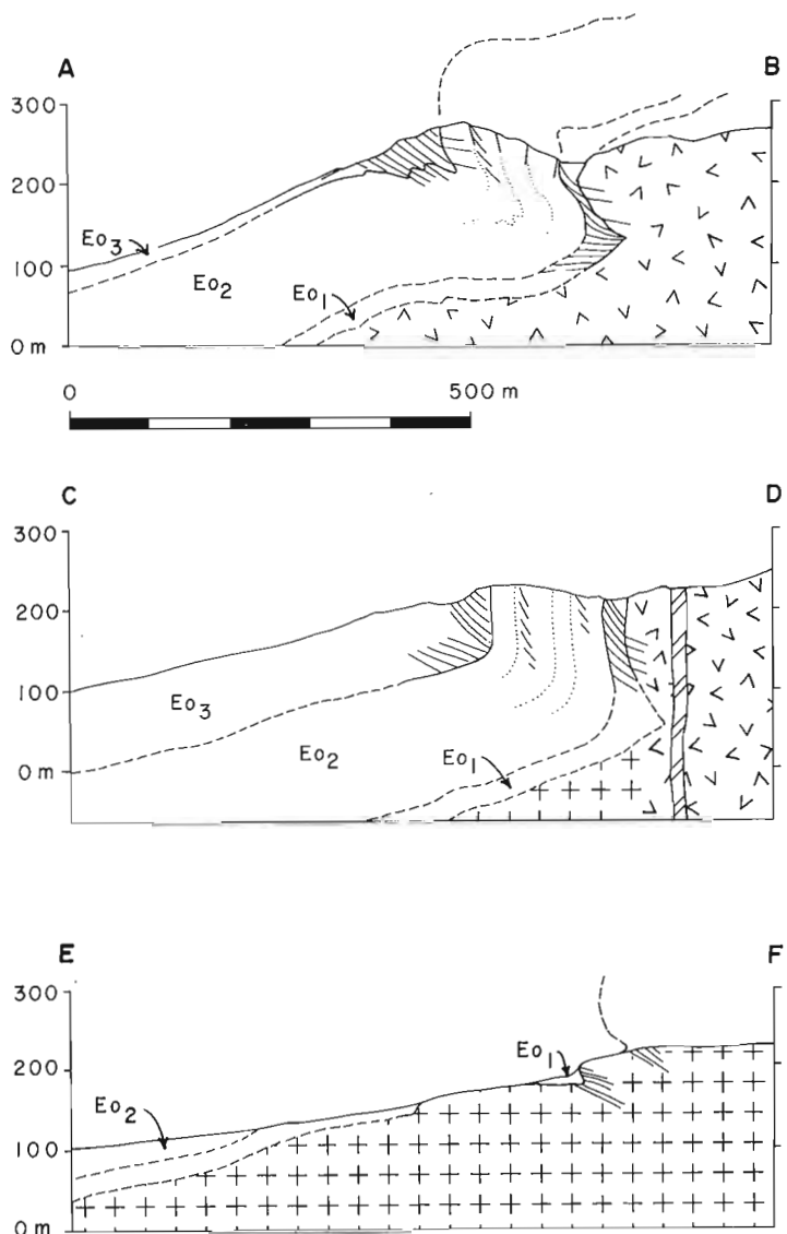
Figure 52.9. Geological map and cross-sections of a part of the western margin of Uyarak Uplift (see Fig. 52.8 for location) showing the cusate-lobate geometry typical of the basement/cover contact in the Tree River Fold Belt. Topographic relief here is great enough for excellent structural control.
