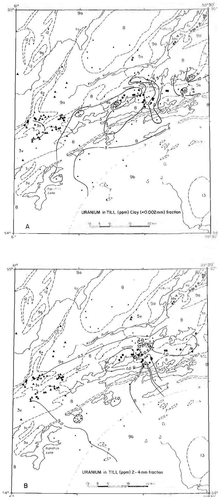
Figure 35.8. Regional variation in the uranium content in the (A) clay-size (<0.002 mm) and (B) pebble-size (2-4 mm) fractions of till. Bedrock geology is explained in Figure 35.1.
