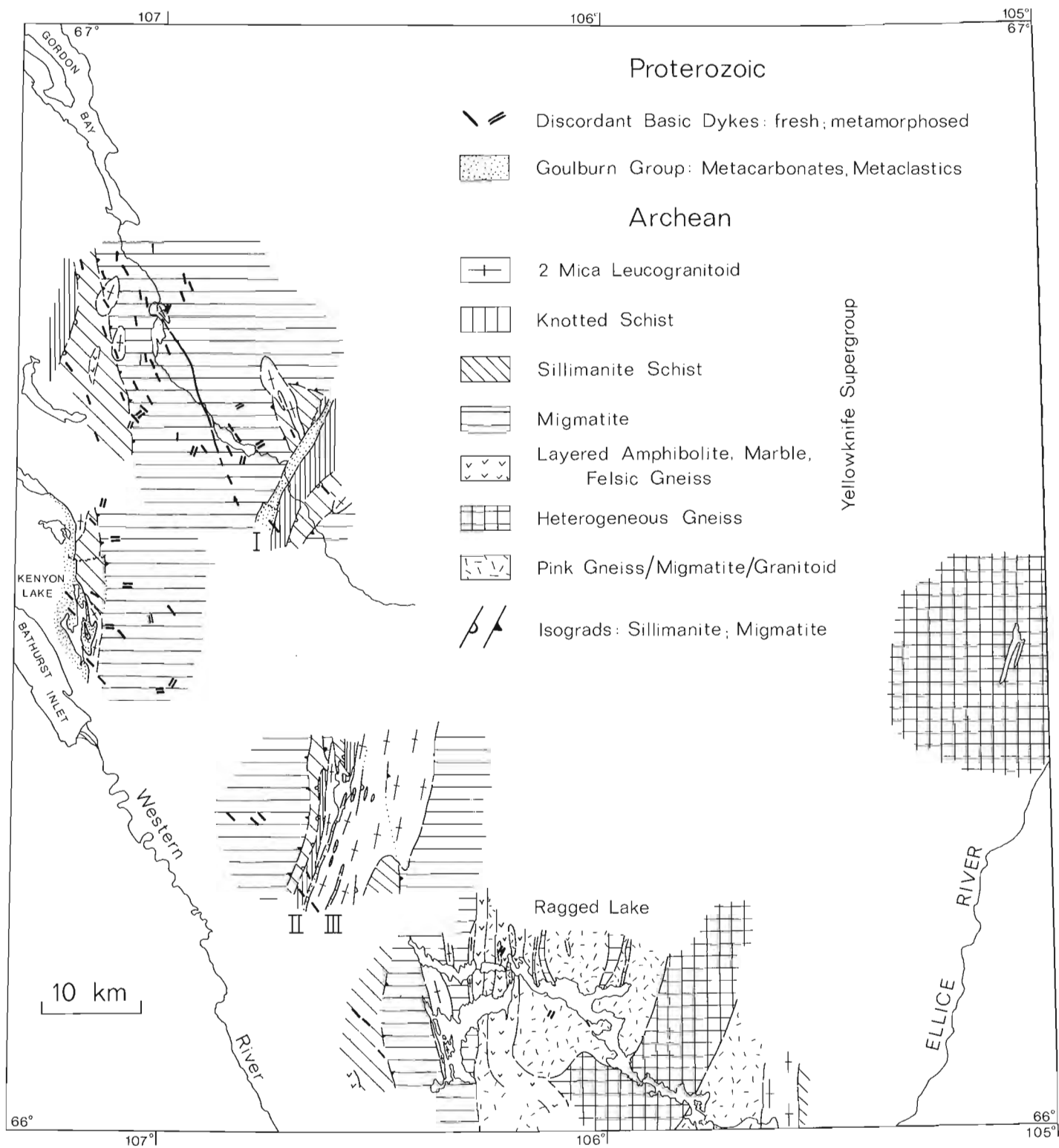
Figure 55.2. Geology of parts of the Tinney Hills-Overby Lake map area. Roman numerals refer to outlines of Goulburn Group.
