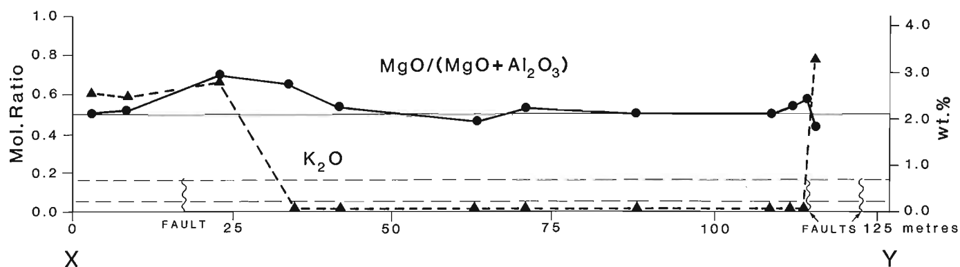
Figure 81.3. Whole rock geochemical traverse across the Mathiati hydrothermal alteration pipe along the X-Y indicated on Figure 81.2, illustration variations in \text{MgO}/(\text{MgO} + \text{Al}_2\text{O}_3) mole ratios (thick solid line) and \text{K}_2\text{O} content (thick broken line). Assumed original values for unaltered rocks are taken from the average of Lower Pillow Lavas (Desmet et al., 1980) and the average of basaltic glasses (Robinson et al., 1983). \text{MgO}/(\text{MgO} + \text{Al}_2\text{O}_3) mole ratios (thin solid line) of both data sets are similar, but average \text{K}_2\text{O} contents (thin broken lines) are 0.76 and about 0.2% respectively.
