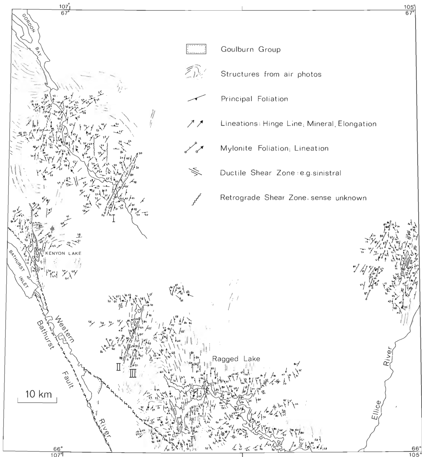
Figure 55.3. Structural trends in parts of the Tinney Hills map area. Roman numerals refer to outliers of Goulburn Group.
