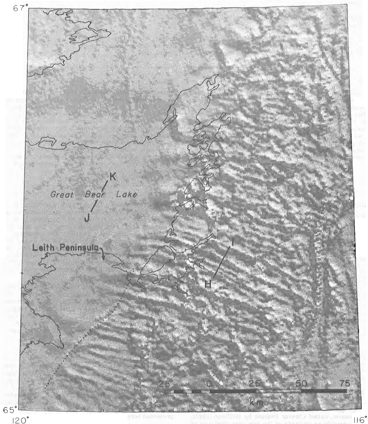
Figure 32.1. Computer-generated shaded-relief magnetic map of the Leith Peninsula area, District of Mackenzie. The original aeromagnetic data were drupe flown at a 300 m terrain clearance along E-W flight lines spaced 800 m apart, and the resultant aeromagnetic maps were digitized at an 812.8 m interval. To enhance the Cleaver Diabase magnetic anomalies, the digitized aeromagnetic data were illuminated using a sun azimuth of 025° and an inclination of 40° above the horizontal. The Cleaver Diabase is represented by the strong linear features which strike 295° and are transected, in part, by line HI. Line HI is situated over Great Bear Magmatic Zone and line JK is along strike of the Cleaver Diabase but over the Hornby Bay Group. The dotted line represents the trace of northeast-trending normal faults bounding the northwest side of Leith Ridge.
