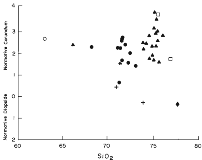
Figure 29.4. Plot of CIPW normative corundum or diopside against \text{SiO}_2 . Symbols are as in Figure 29.3, except mean values are indicated by asterisk (Deep Cove granite), diamond (Petit de Grat leucogranite), and crosses (Huntington Mountain quartz monzonite and leucogranite).
