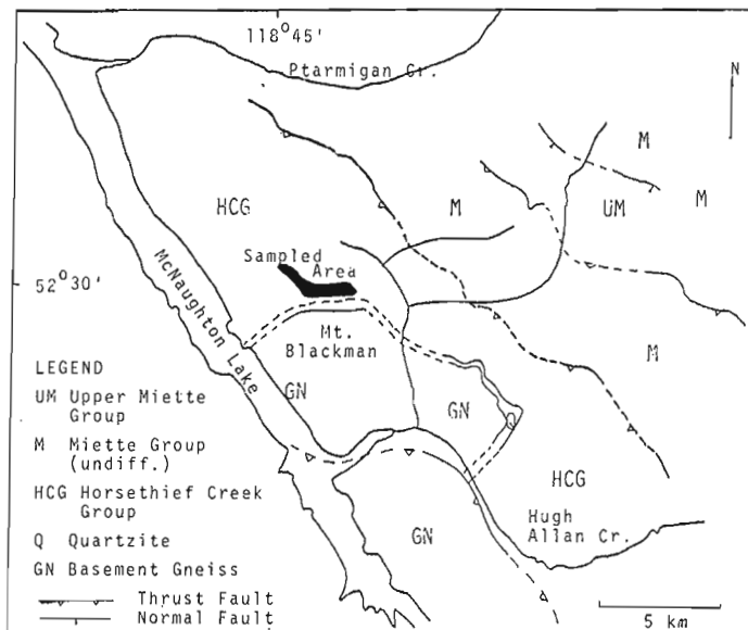
Figure 20.1. Geology around Mount Blackman, British Columbia.
