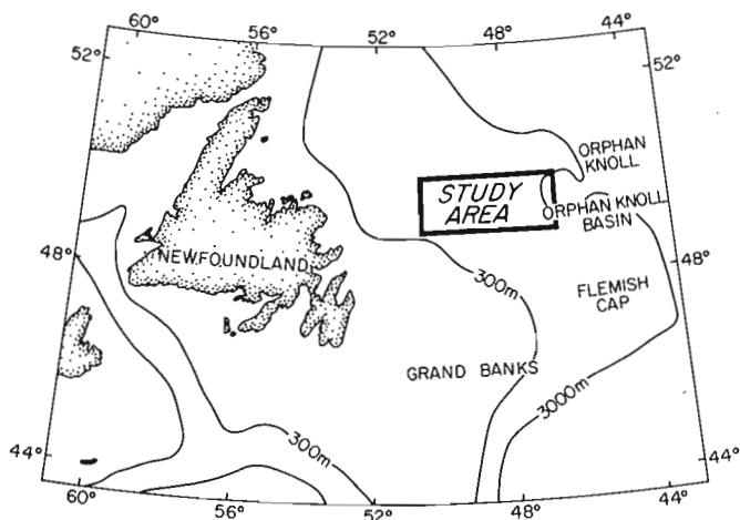
Figure 75.1. Location of the study area on the northeast Newfoundland continental slope and rise showing its position relative to the 300 and 3000 m isobaths.
