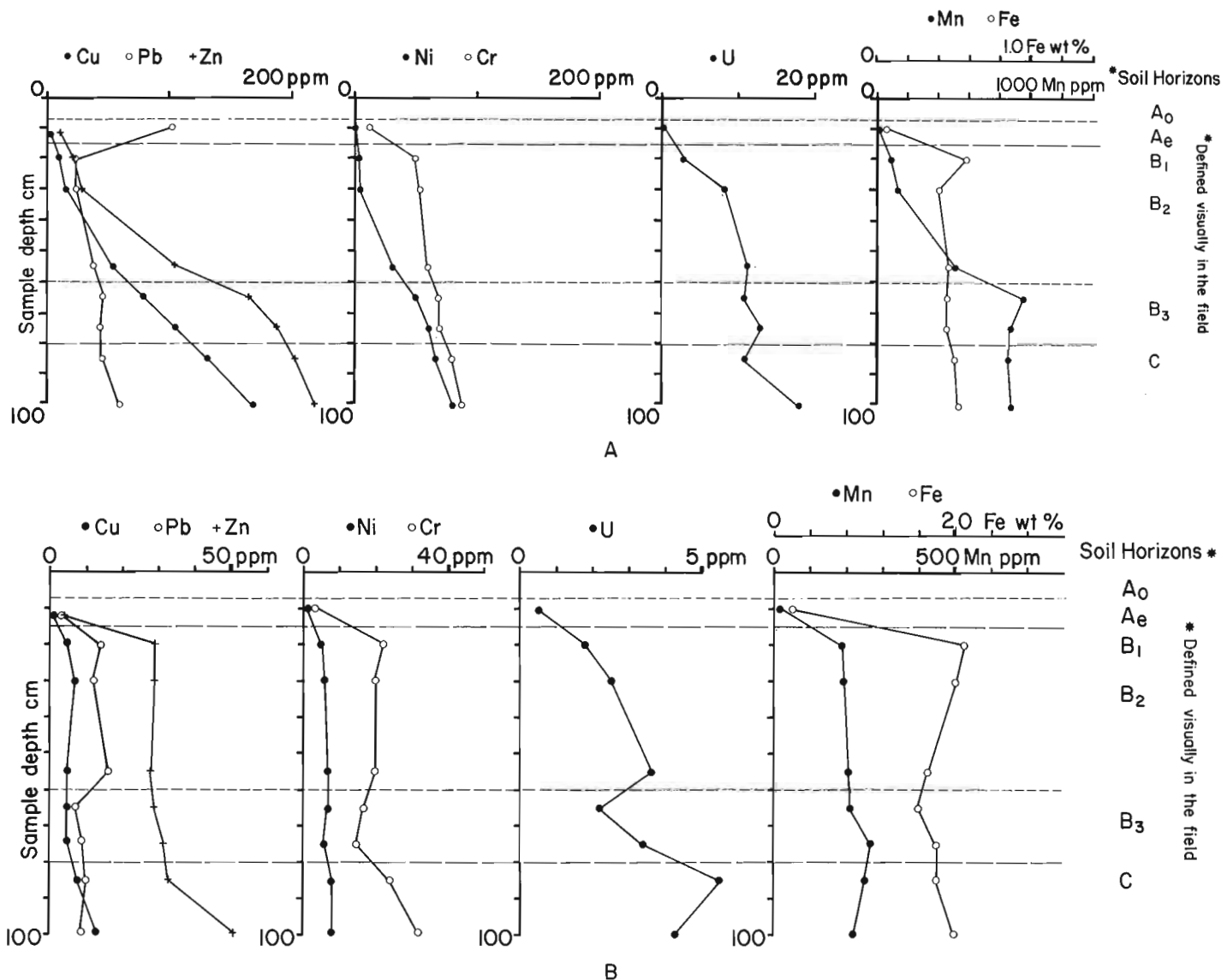
Figure 35.5. Trace element variation in (A) clay-size (<0.002 mm) and (B) pebble-size (2-4 mm) fractions within the soil profile shown in Figure 35.4. The pit was dug within a dispersal train of uraniferous erratics, and metal contents are generally greater than found elsewhere in the study area. The shapes of the trace element profiles are, however, typical.
