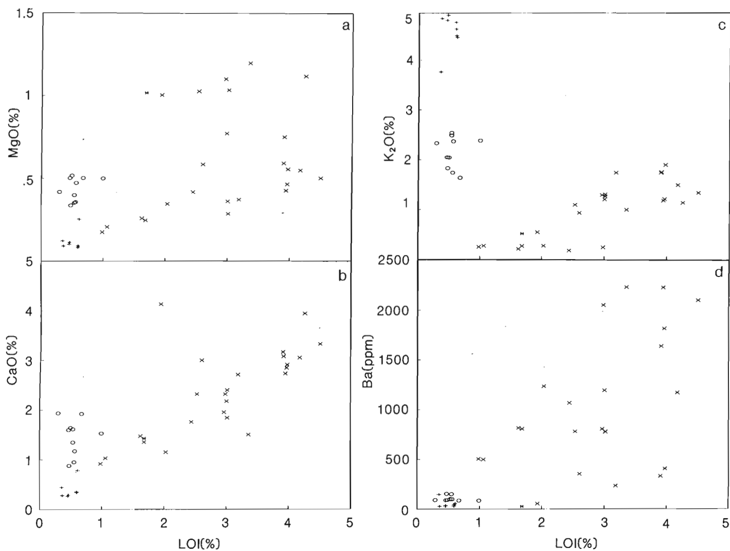
Figure 62.3. Diagrams illustrating the effects of alteration on particular elements: a) loss on ignition (LOI) vs MgO; b) LOI vs CaO; c) LOI vs \text{K}_2\text{O} ; d) LOI vs Ba. For symbols see Figure 62.1.
