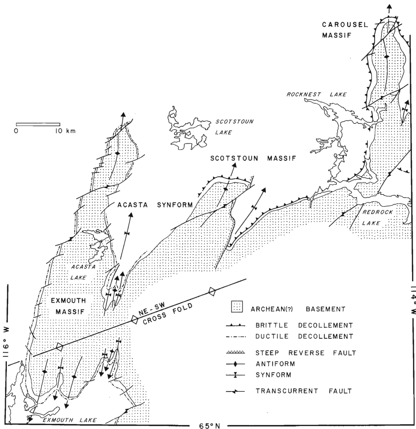
Figure 25.1. Location of the three basement massifs and the regional décollement as exposed by a major northeast-southwest cross fold.
