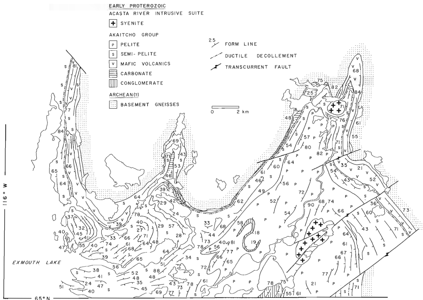
Figure 25.2. Major stratigraphic units of the Akaitcho Group with the ductile decollement, and form lines in both high and low strain domains east of Exmouth Lake.
