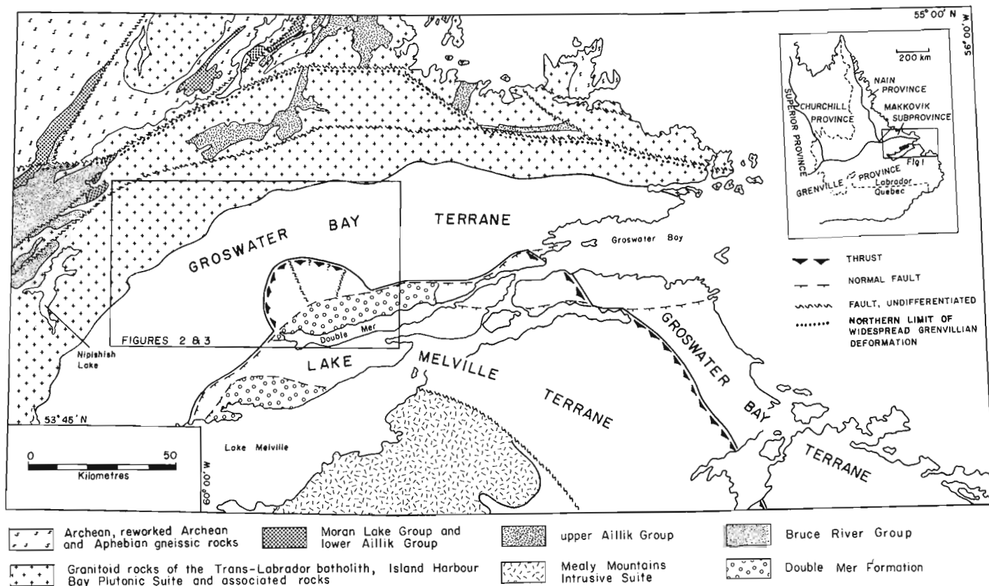
Figure 74.1. Regional geological subdivision of the Grenville structural province in eastern Labrador.
