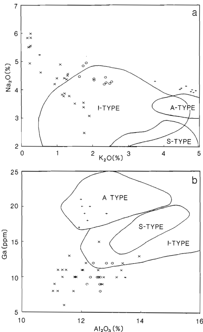
Figure 62.1. Discriminant diagram for granitoid magma series from White and Chappell (1983): a) K 2 O vs Na 2 O; b) Al 2 O 3 vs Ga. The (x) represents a granitoid clast sample from MacLean Extension orebody, (o) represents a Feeder Granodiorite sample, the (+) represents the Topsail (alkali feldspar) granite sample, and the (*) represents the sample from the Little Sandy intrusion.
