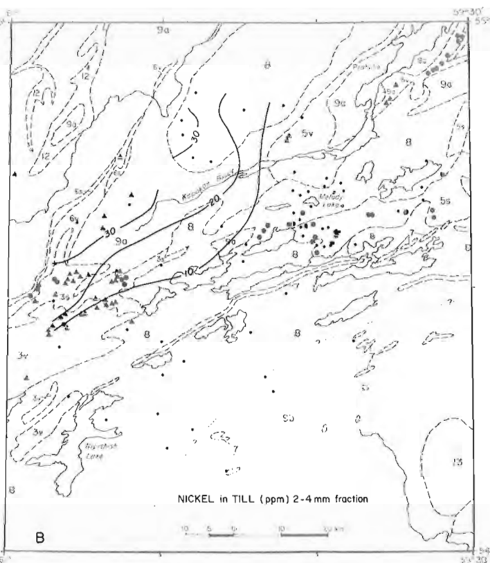
Figure 35.7. Regional variation in the nickel content in the (A) clay-size (<0.002 mm) and (B) pebble-size (2-4 mm) fractions of till. Bedrock geology is explained in Figure 35.1.
