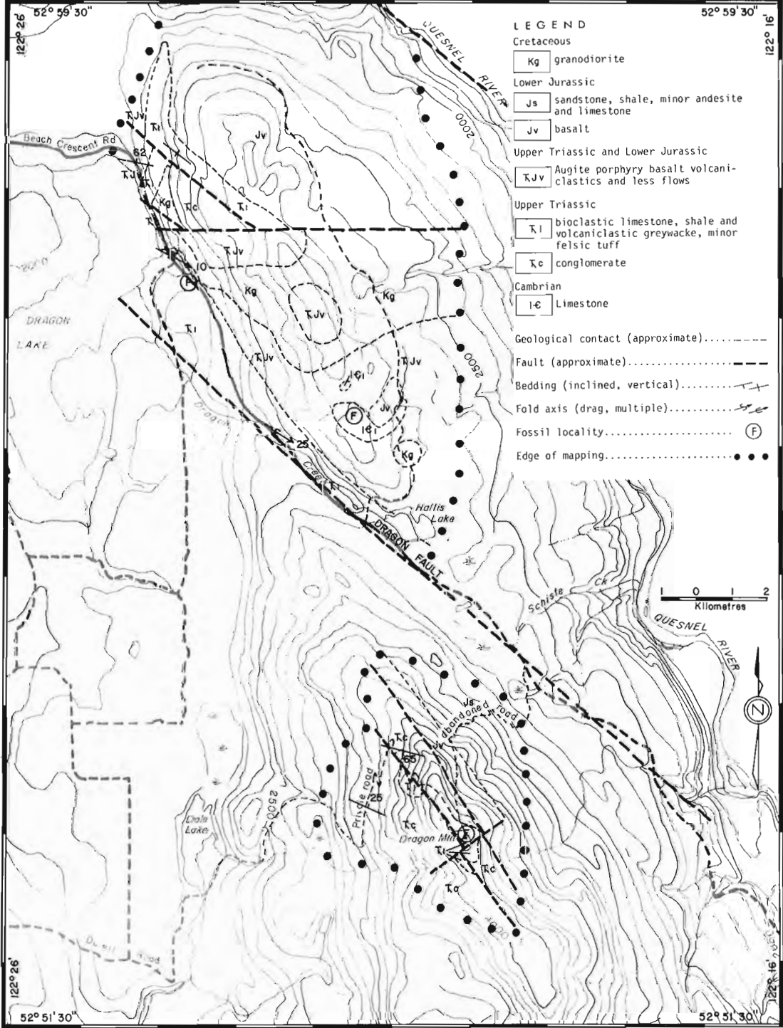
Figure 18.2. Geological map of the study area. Located in Figure 18.1C.
