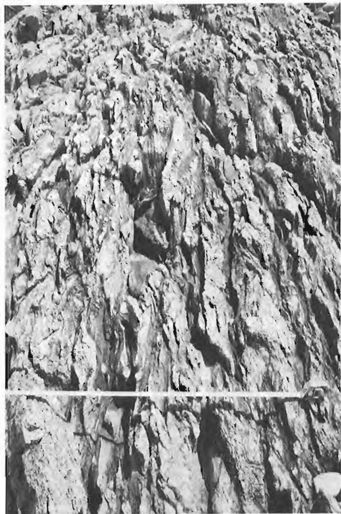
Figure 22.4. Flattened intraformational conglomerate: angular slate clasts (dark) surrounded by a matrix of very coarse sand and granule-size material, Outer Island. Scale is 1 metre.
