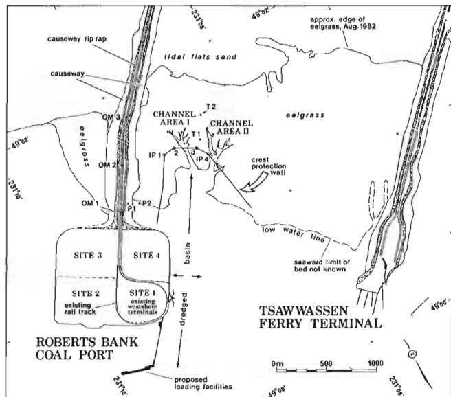
Figure 9.2. Major features within study area including dendritic channel system at head of dredged ship basin (arrows within basin denote approximate dimension in 1970). OM, P, IP represent survey marker locations. T = navigation towers. Adapted from National Airphoto Library imagery (Roll #A37849) and Swan Wooster Engineering Co. Ltd. blueprint drawings.
