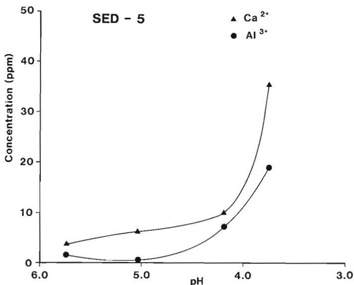
Figure 79.5. Liberation of \text{Ca}^{2+} and \text{Al}^{3+} into solution during acidification of sample SED-5.
