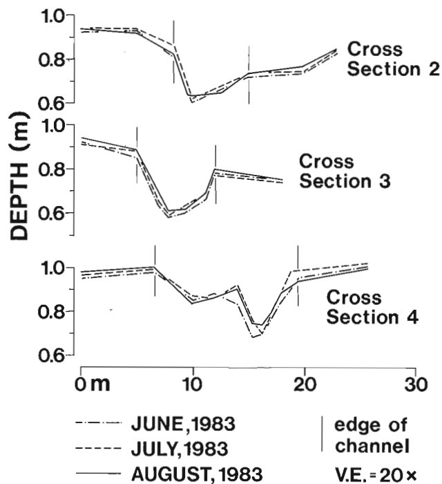
Figure 9.5. Comparison of channel profiles surveyed in channel area I (Fig. 9.3; profile locations 2, 3, 4).
