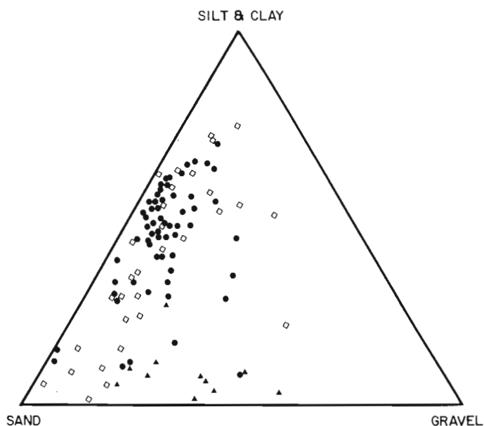
Figure 46.2. Triangular diagram showing the general grain size distributions of diamictons on Somerset Island. Squares represent weathered rock diamictons; triangles are grus; large dots are tills.
