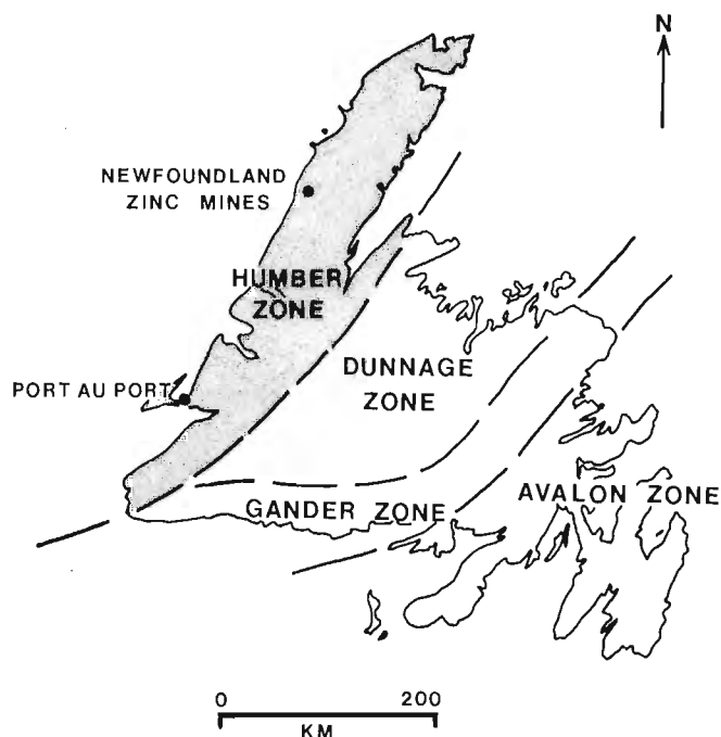
Figure 68.1. Tectono-stratigraphic zones of Newfoundland with the location of Newfoundland Zinc Mines (after Williams, 1979).
