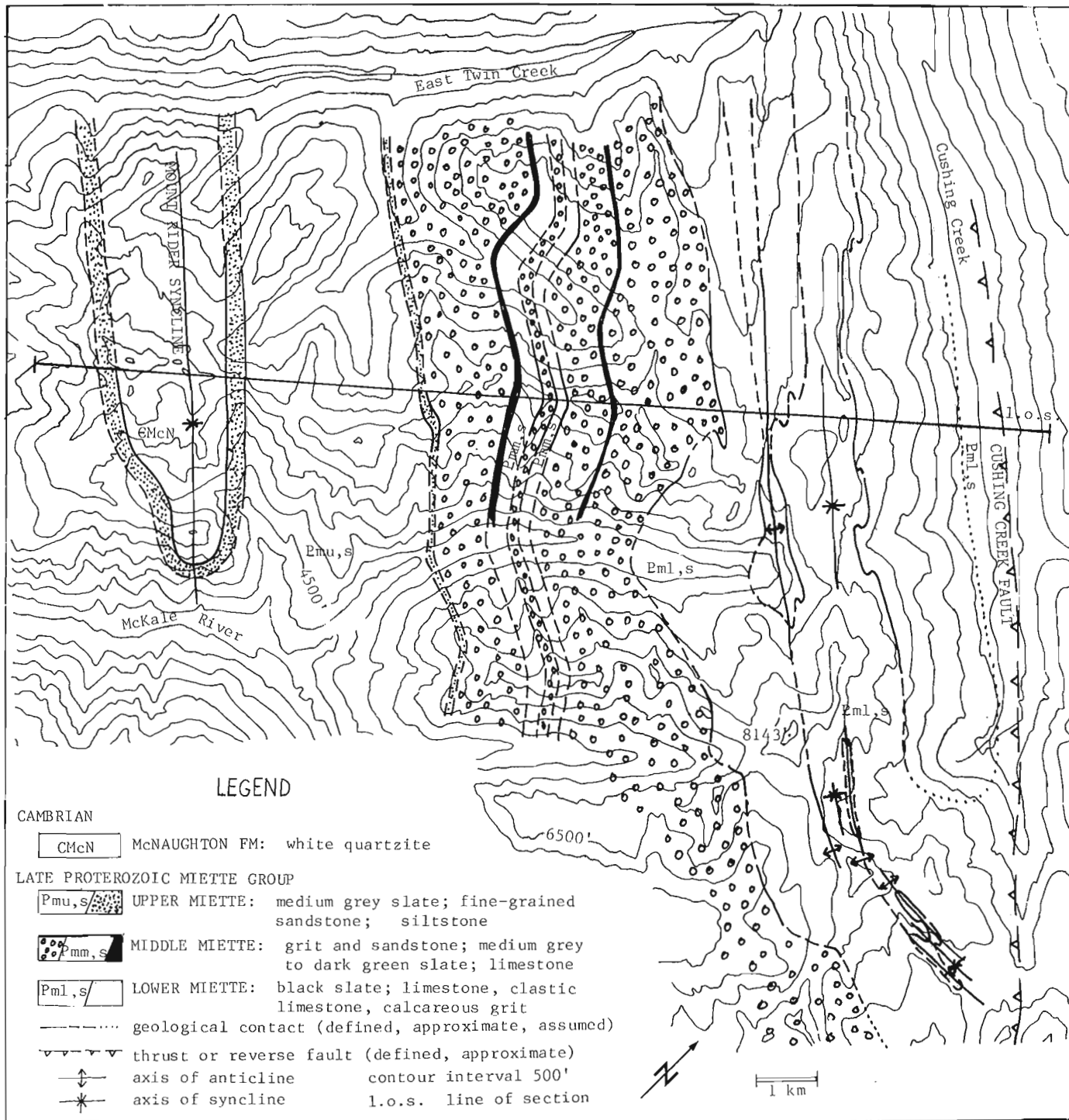
Figure 56.2. Geological map of study area.
