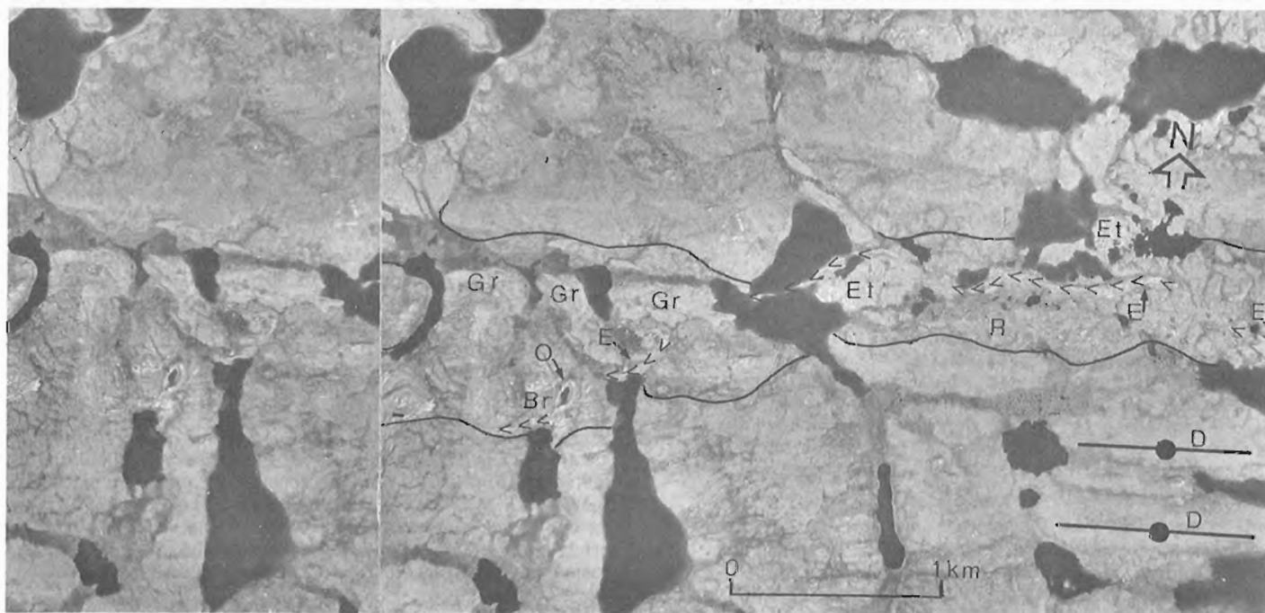
Figure 38.3. Stereogram of glaciofluvial corridor and associated landforms. E, esker; Et, esker terrace; Gr, gravel and sand; O, oval ridge (Fig. 38.4, 38.5); Br, bedrock; R, minor ridges. Note well developed drumlins (D) typical of Irritation Lake drumlin field. NAPL A11532-135, 136.
