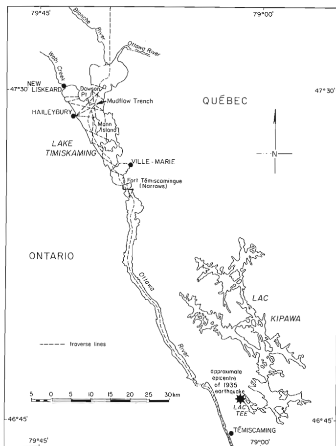
Figure 76.2. Location map of Lac Tee - Lake Timiskaming region. Mudflow trench is the site of profiles in Figure 76.9. Dashed lines are traces of some of the sonar profiles.
