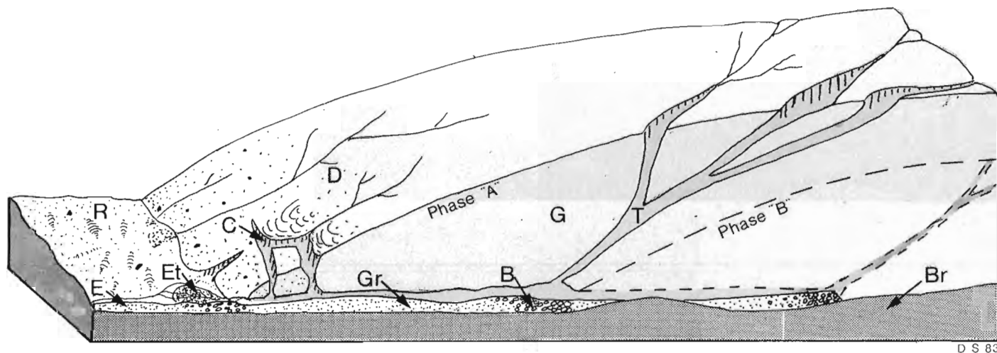
Figure 38.2. Origin of sediments and associated landforms along a glaciofluvial corridor. Note that during phase B the constricted flow above a bedrock knob prevents sedimentation; this will result in a "washed surface". E, esker; Et, esker terrace; Gr, gravel and sand; B, boulders; R, ridges; C, crevasses; D, debris; G, glacier ice; T, tunnel; Br, bedrock.
