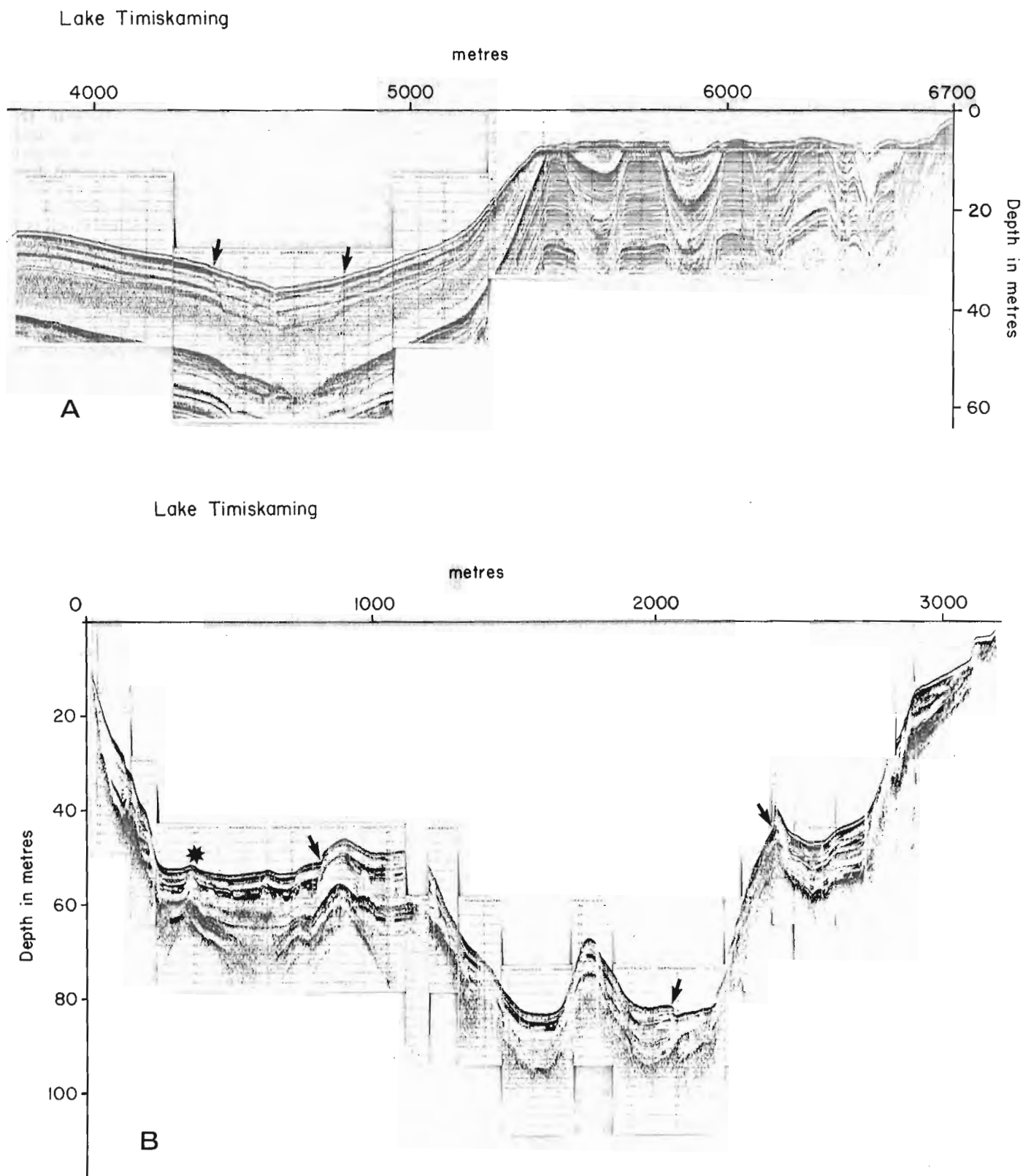
Figure 76.10. Faulting of modern sediment in Lake Timiskaming. A. Faulting (arrows) in thick, modern sediment just south of the mudflow trench north of Mann Island. B. Faulting (arrows) and possible diapirism (*) in a deep trench near the narrows.
