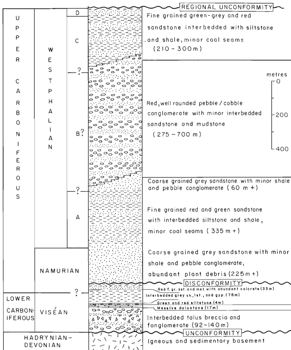
Figure 2 General stratigraphy of the Glengarry Half Graben.
