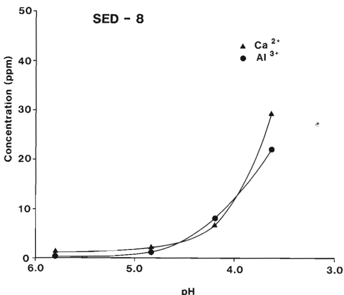
Figure 79.6. Liberation of \text{Ca}^{2+} and \text{Al}^{3+} into solution during acidification of sample SED-8.
