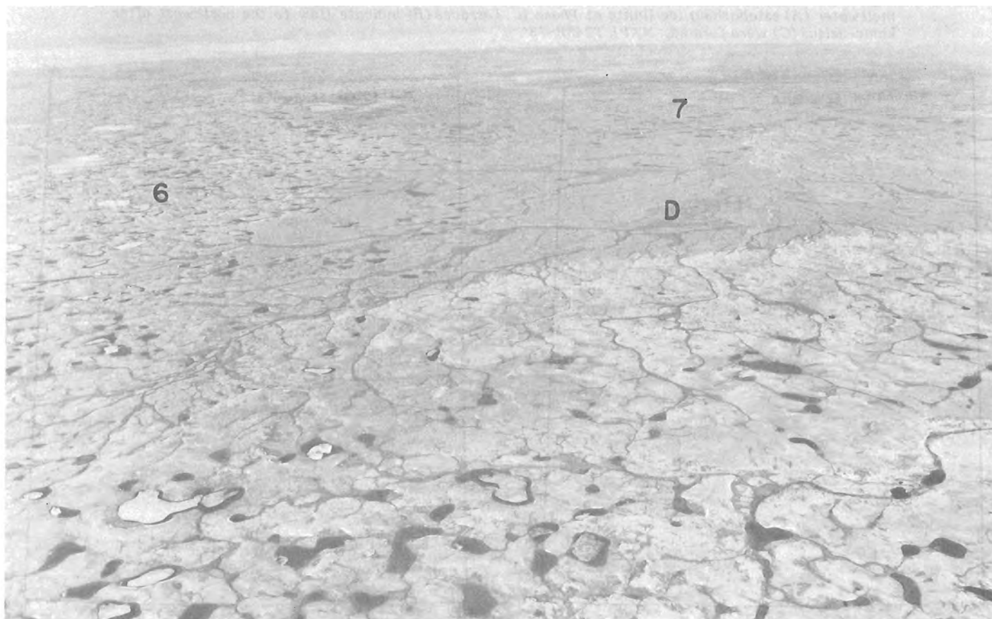
Figure 37.11. View to west across zone 7 terrain (Fig. 37.2, ground moraine) showing well developed outwash system (D) indicating open drainage to the west during formation of large areas of hummocky moraine as landform zone 6. NAPL T330L-108
