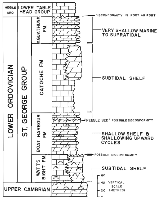
Figure 71.2. Schematic stratigraphic section of the Lower Ordovician St. George Group. Proposed depositional environments (in heavy type) and the locations of disconformities within the St. George Group are summarized on the right side of the section. Coarsely crystalline dolomitization of parts of the Watts Bight and Catoche formations are indicated by the cross hatched pattern. (Data from Knight, 1977b, 1978).
