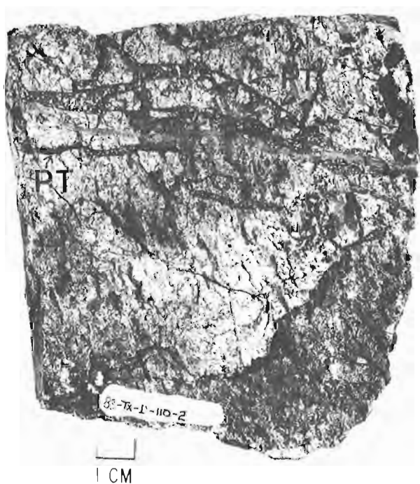
Figure 43.11. Breccia zones with pseudotachylite fractions cutting mylonitic layering; Chantrey Mylonite Zone. GSC 203308-V
