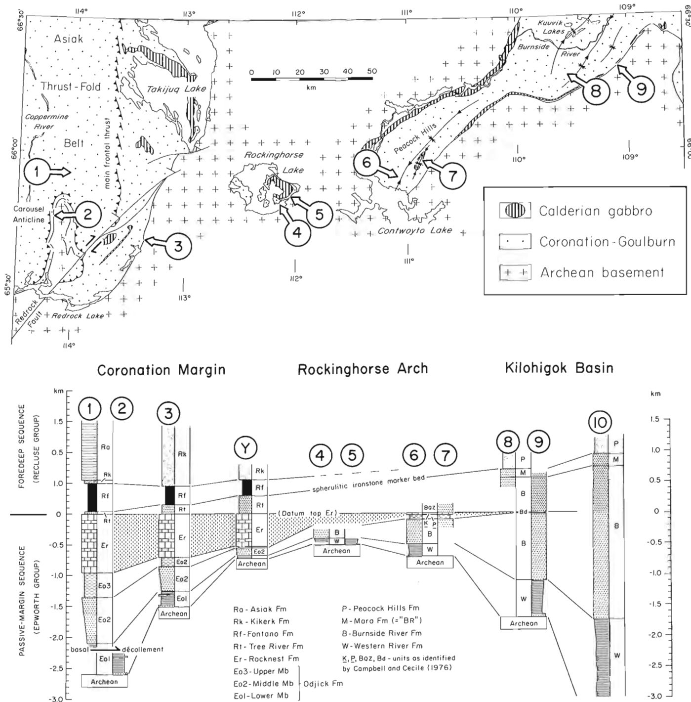
Figure 52.6. Location of sections and proposed correlation of the Rocknest Formation across Rockinghorse Arch into Kilohigok Basin. Section "Y" is located in the Tree River Fold Belt (see Fig. 52.1) and section 10 is a composite from around Bathurst Inlet.
