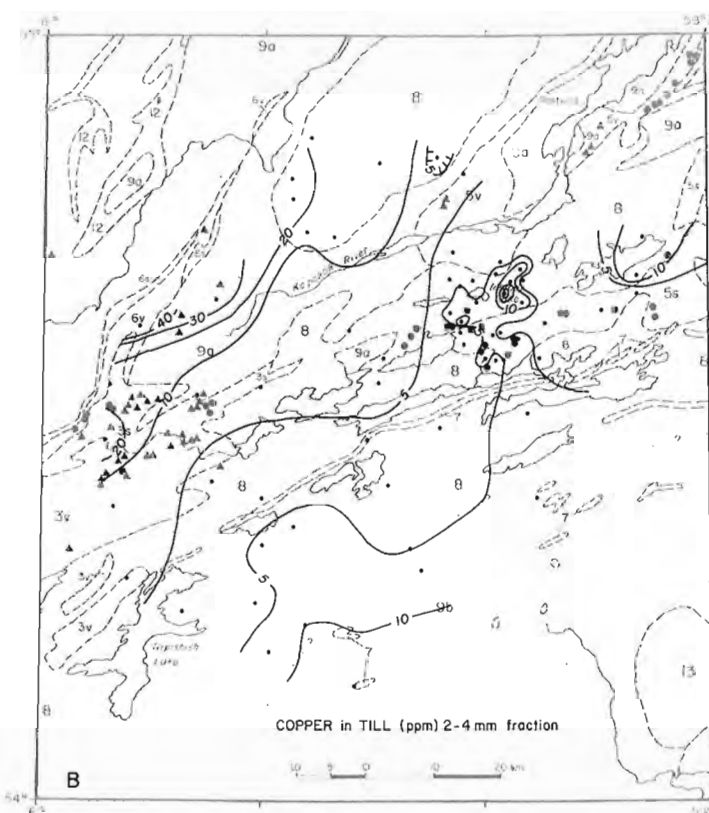
Figure 35.6. Regional variation in the copper content in the (A) clay-size (<0.002 mm) and (B) pebble-size (2-4 mm) fractions of till. Bedrock geology is explained in Figure 35.1.
