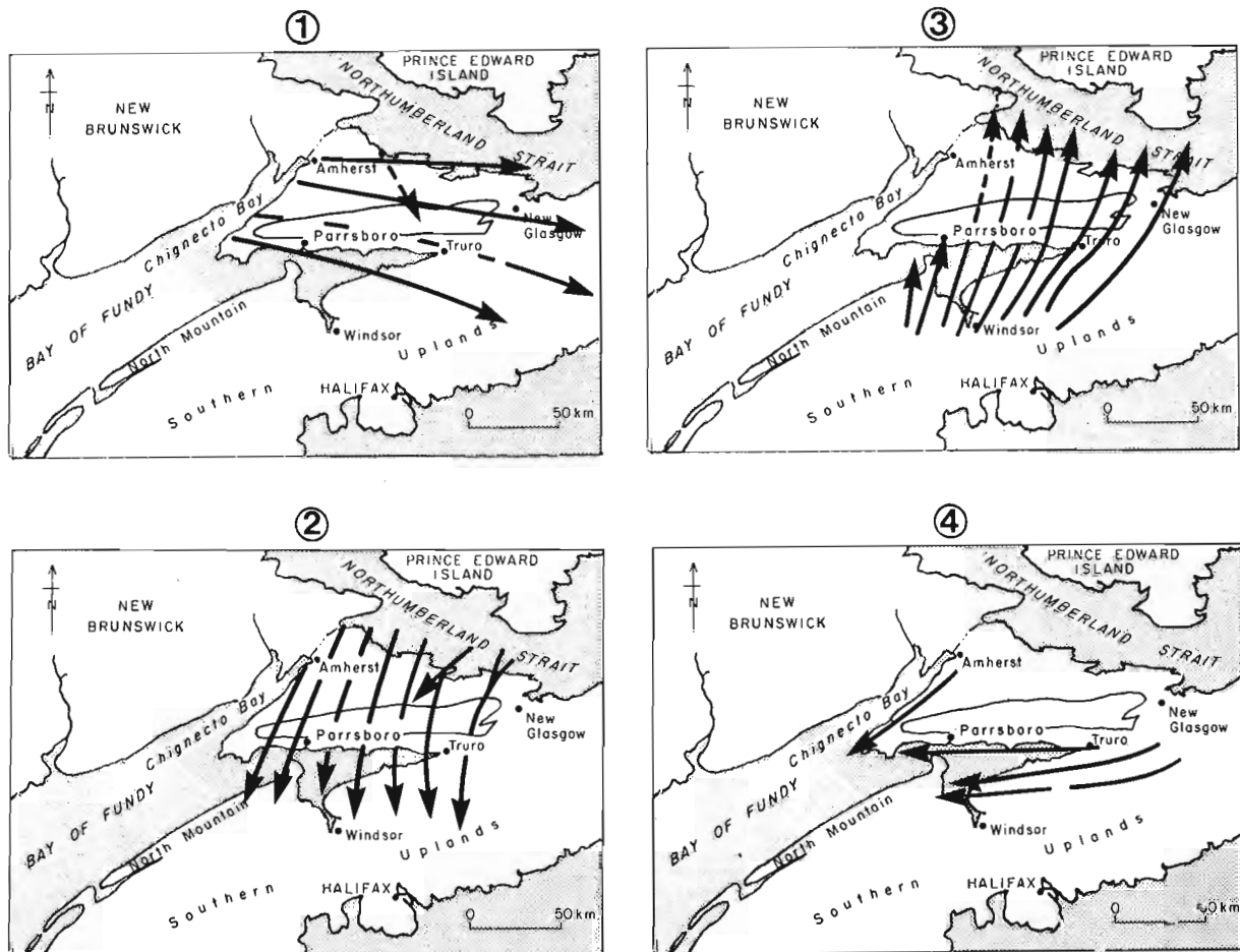
Figure 64.10. The inferred sequence of ice flows in the map area. Flow pattern 1 is speculated to be Early Wisconsin in age; flow patterns 3 and 4 Late Wisconsin.
