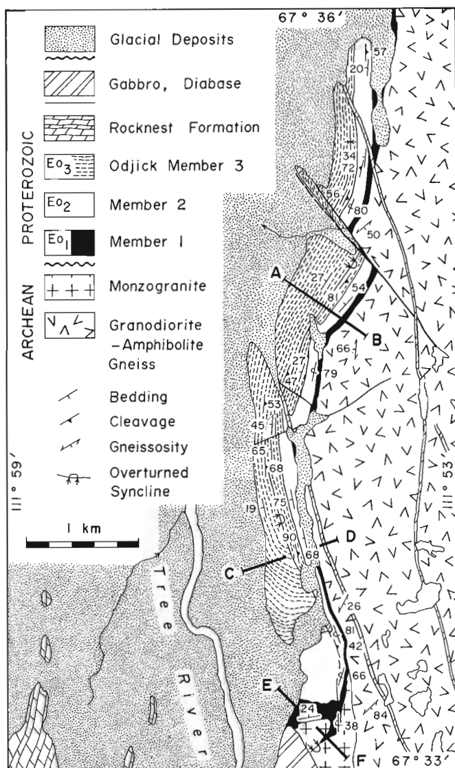
Figure 52.9. Geological map and cross-sections of a part of the western margin of Uyarak Uplift (see Fig. 52.8 for location) showing the cusate-lobate geometry typical of the basement/cover contact in the Tree River Fold Belt. Topographic relief here is great enough for excellent structural control.
