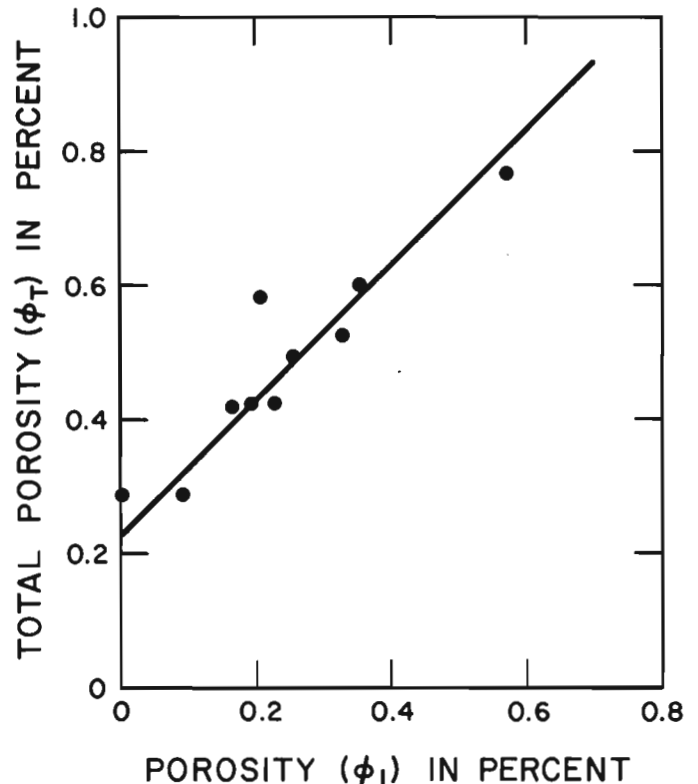
Figure 4.9. Total porosity ( \phi_T ) plotted against porosity ( \phi_1 ) of first component. For statistics, see Table 4.3. Straight line with equation \phi_T = \text{constant} + \phi_1 was fitted by method of least squares to all values except "outlier" for WN1-410.
