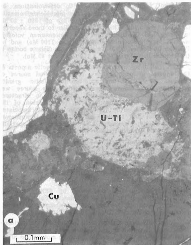
Figure 5.4a,b. Mineral assemblage in the matrix of the conglomerate from the upper portion of the Matinenda Formation, at the south shore of Elliot Lake, Ontario. Zr = zircon, U-Ti = Ti-U-Si-Fe phase, Cu = chalcopyrite, Cr = chromite. Photomicrograph, reflected light.
