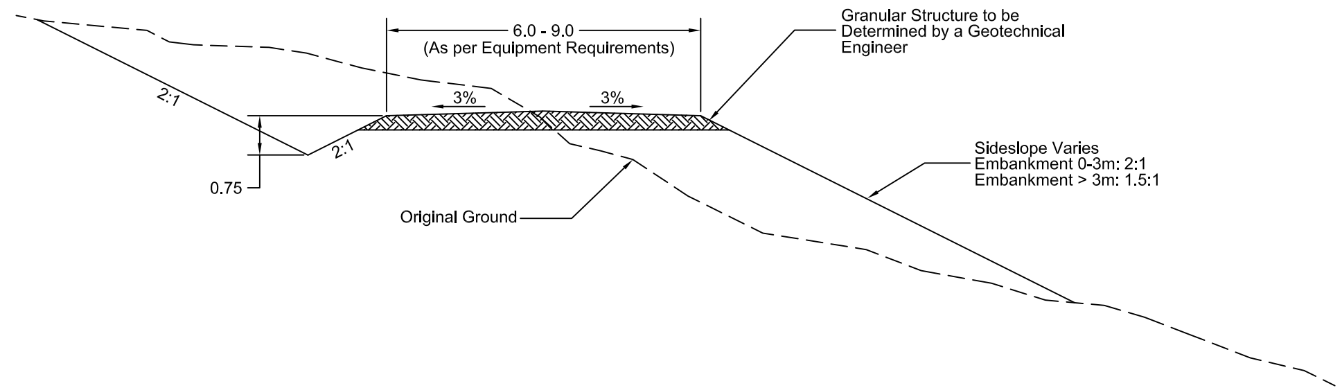
Typical Cross-Section Access Road
