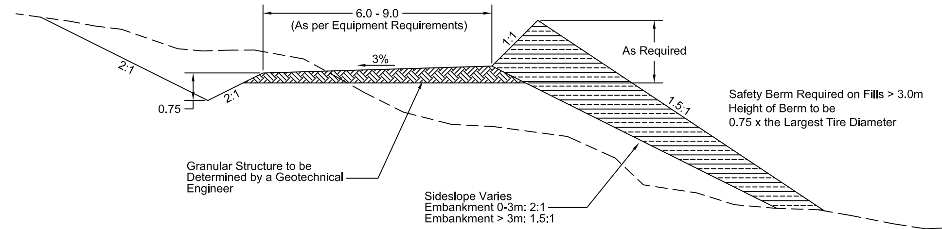
Typical Cross-Section - Safety Berm Haul Road
