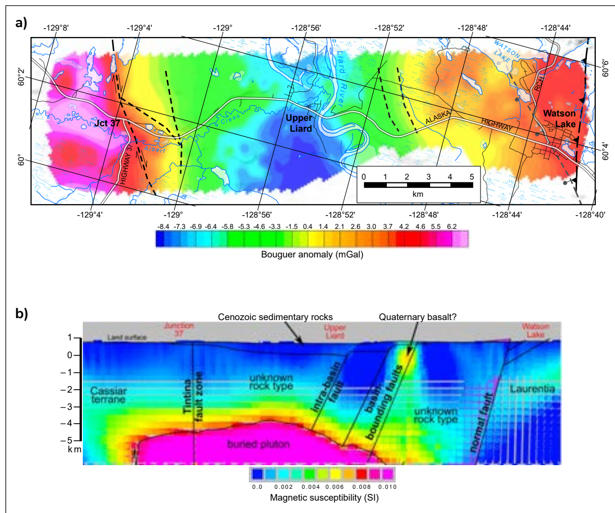
Figure 37. a) Bouguer gravity anomaly map for density of 2.67 g/cm 3 with upward continued 2500 m trend removed (Aurora Geosciences, adapted from Witter, 2022). RCH: Robert Campbell Highway. b) Section through 3D magnetic inversion model along the Alaska Highway corridor near Watson Lake (modified from Witter, 2022). A strong magnetic anomaly straddling the western part of the Tintina fault zone is modelled to represent a possible pluton at depth of >4 km below sea level.
