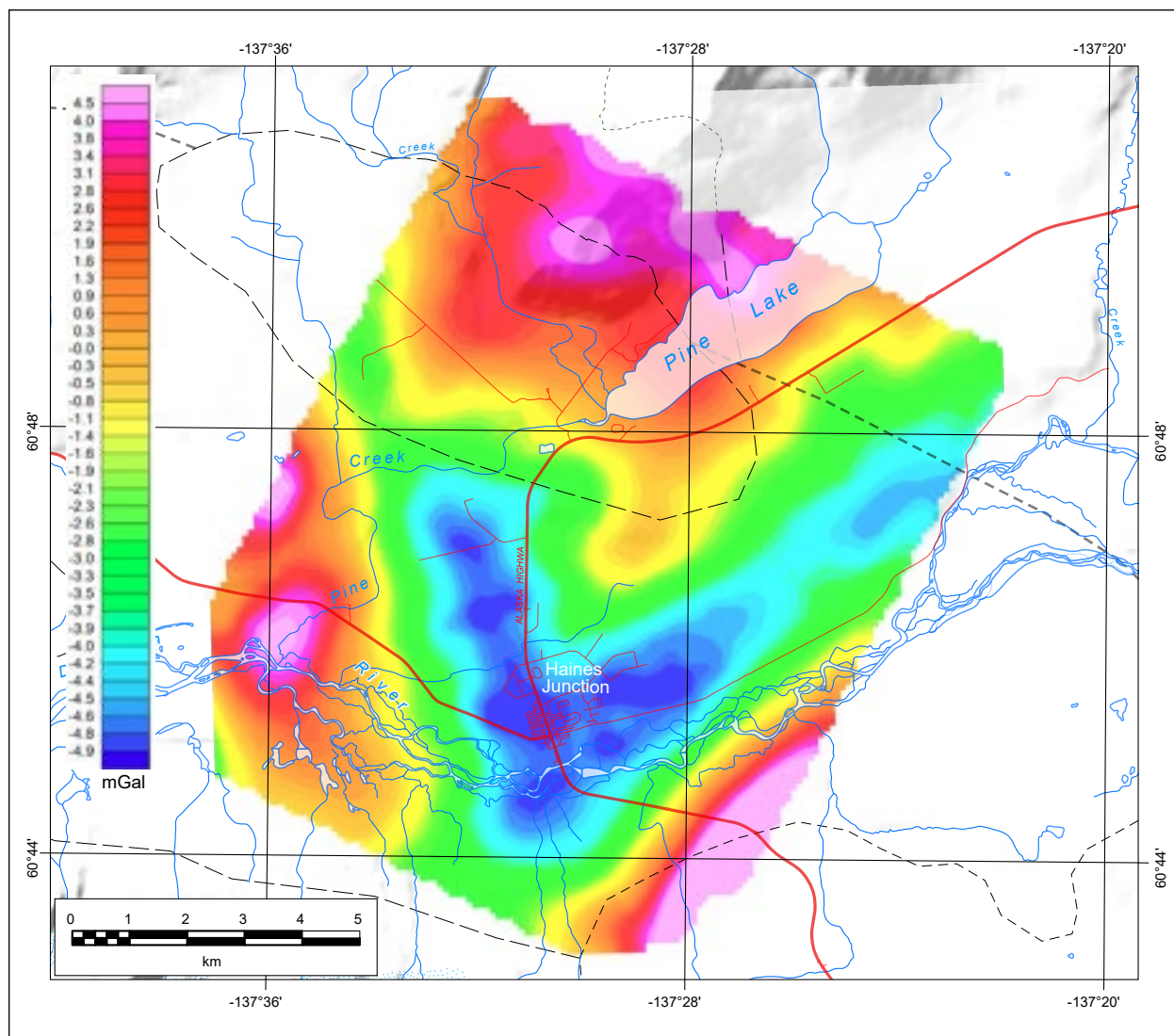
Figure 61. Bouguer gravity anomaly map for a density of 2.67 \text{ g/cm}^3 with upward continued 2500 m trend removed (adapted from Witter, 2024).
