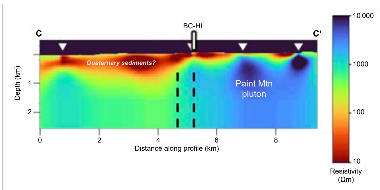
Figure 62. Section through a 3D resistivity model based on broadband magnetotelluric data for the Haines Junction (Dakwǎkǎda) area (C. Hanneson, pers. comm., 2024). The location of the section is indicated on Figure 60. Note that depth is relative to the elevation at Haines Junction (Dakwǎkǎda; ~600 m above sea level). The strong resistivity in the northern part of the section (towards C') corresponds to the crystalline rocks of the Paint Mountain pluton (Hayden Lake suite). Strong near-surface conductivity likely reflects Quaternary sediment fill in the area. BC-HL indicates the approximate location of the contact between the Bear Creek assemblage (BC) and the Paint Mountain pluton (HL: Hayden Lake suite).
