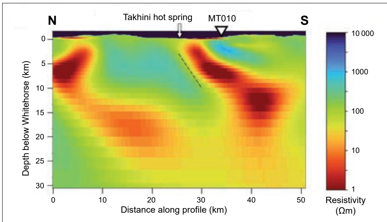
Figure 49. Section through a 3D resistivity model from broadband magnetotelluric data highlighting a strong resistivity contrast beneath Takhini hot spring, Yukon (C. Hanneson, pers. comm., 2024). The location of this section is shown in Figure 46.
