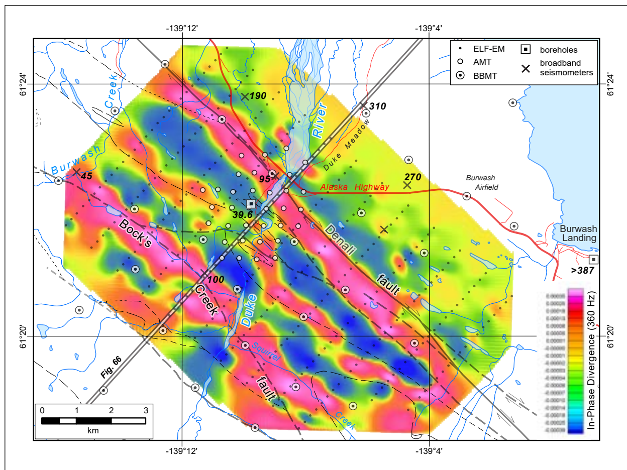
Figure 65. Extremely low frequency electromagnetic (ELF-EM) survey for the Burwash Landing area (adapted from Witter, 2020). In-phase divergence at 360 Hz. The ELF-EM grid is shown with small grey dots; audiomagnetotelluric (AMT) sites are indicated by white circles; broadband magnetotelluric (BBMT) sites by white circles with black dot. Bold-italic numbers show bedrock depth estimates (in metres) derived from shear-wave velocity models created from broadband seismometer readings (Berumen-Borrego et al., 2024) and measured in the two boreholes.
