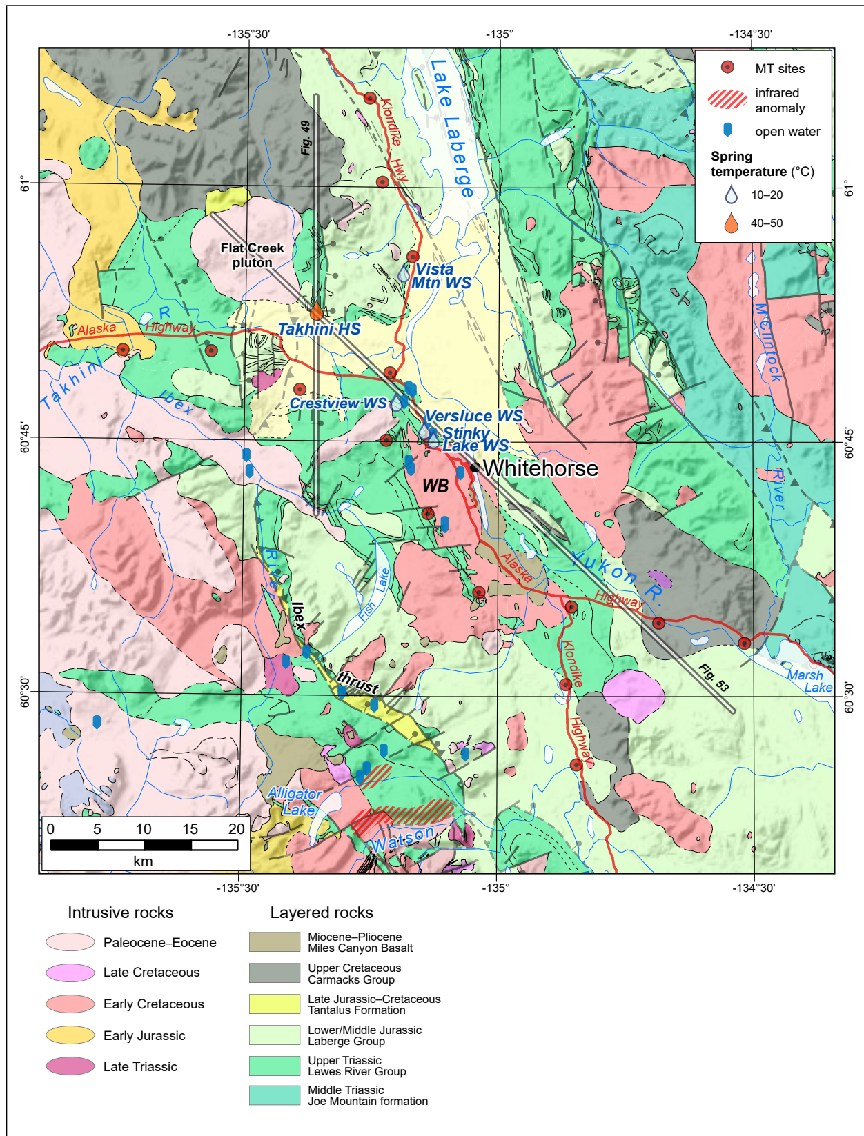
Figure 46. Geology of the Whitehorse area (after Yukon Geological Survey, 2022). The locations of thermal springs, open water and infrared anomalies are indicated. Broadband magnetotelluric (BBMT) sites are shown as red dots. Section lines for the 3D resistivity models shown in Figures 49 and 53 are indicated. HS: hot spring, WB: Whitehorse batholith, WS: warm spring.
