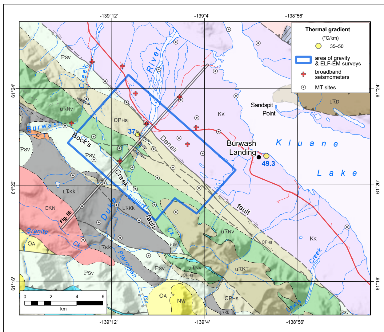
Figure 64. Geology of the Burwash Landing area (Yukon Geological Survey, 2022). The area covered by gravity and extremely low frequency electromagnetic (ELF-EM) surveys (Fig. 65), magnetotelluric (MT) sites, and broadband seismometer locations are shown. The section line for the inversion profile shown in Figure 66 is also indicated.
