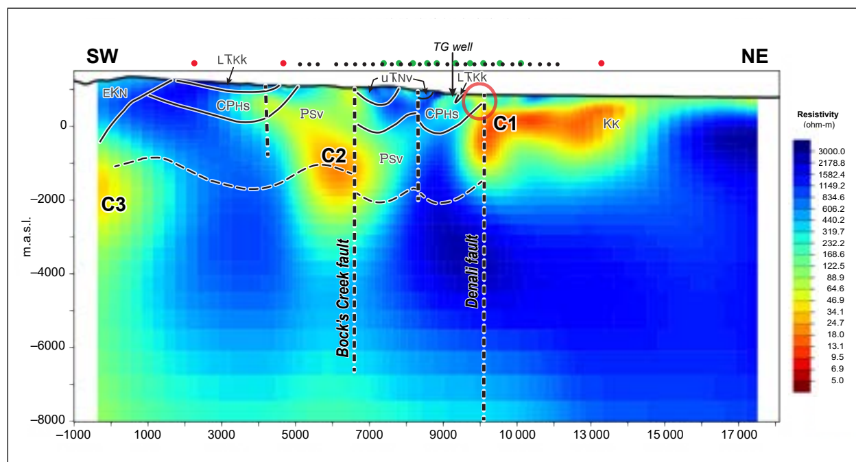
Figure 66. Cross section through the preferred 3D resistivity model from the joint inversion of extremely low frequency electromagnetic (black dots at top of profile), audiomagnetotelluric (green dots) and broadband magnetotelluric (red dots) data (modified from Tschirhart et al., 2022a). C1–C3 are prominent conductors. The red circle highlights a thin conductor emanating from C1 and extending to the surface. A thermal gradient (TG) borehole located on the section is indicated. The location of the section is shown on Figures 64 and 65.
