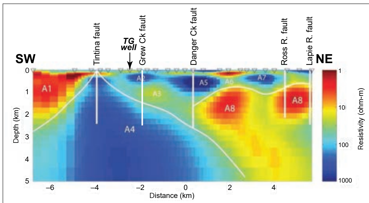
Figure 34. Section through the 3D resistivity model derived from MT data collected by Mira Geoscience (2017). The approximate line of the section is indicated on Figure 33. The strong resistivity of feature A4 suggests the presence of crystalline rocks (granitoid?) at depth northeast of the Tintina fault. Conductive features A1 and A8 likely indicate presence of graphitic rocks, though A8 could also be due in part to aqueous fluids.
